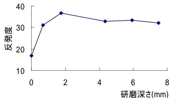
図1 研磨深さの反発度
